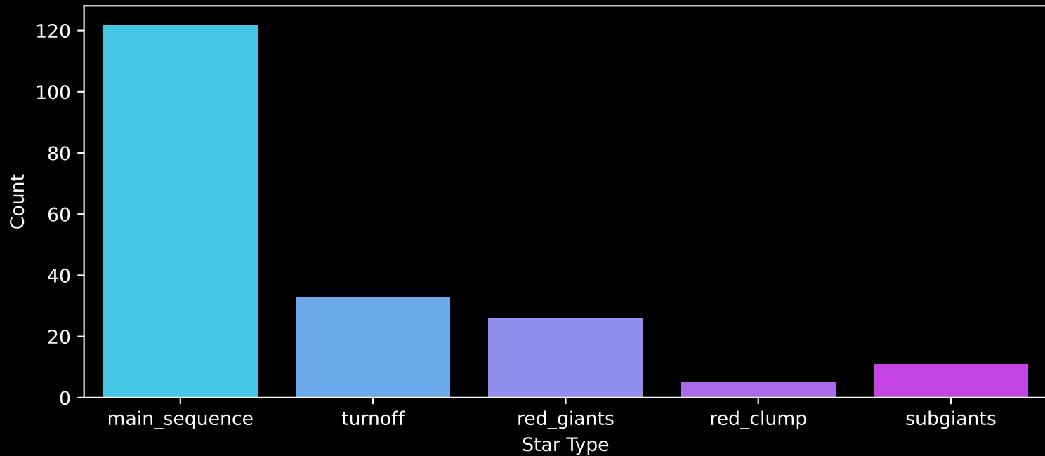
APOGEE DR17 Field: [068+51_MGA] Count plot of Star Type
