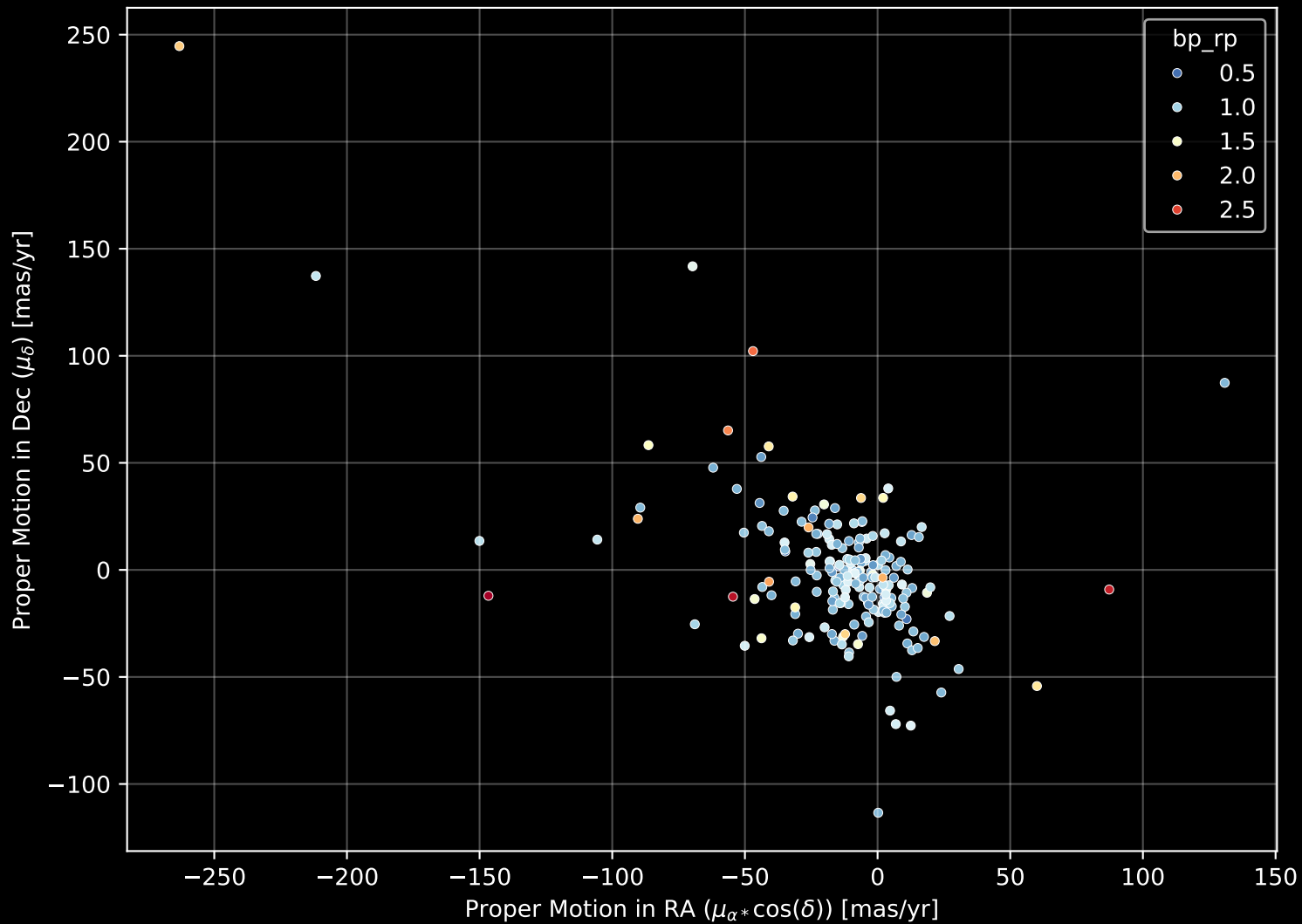
APOGEE DR17 Field: [068+51_MGA] Proper Motion Diagram (n= 197)
