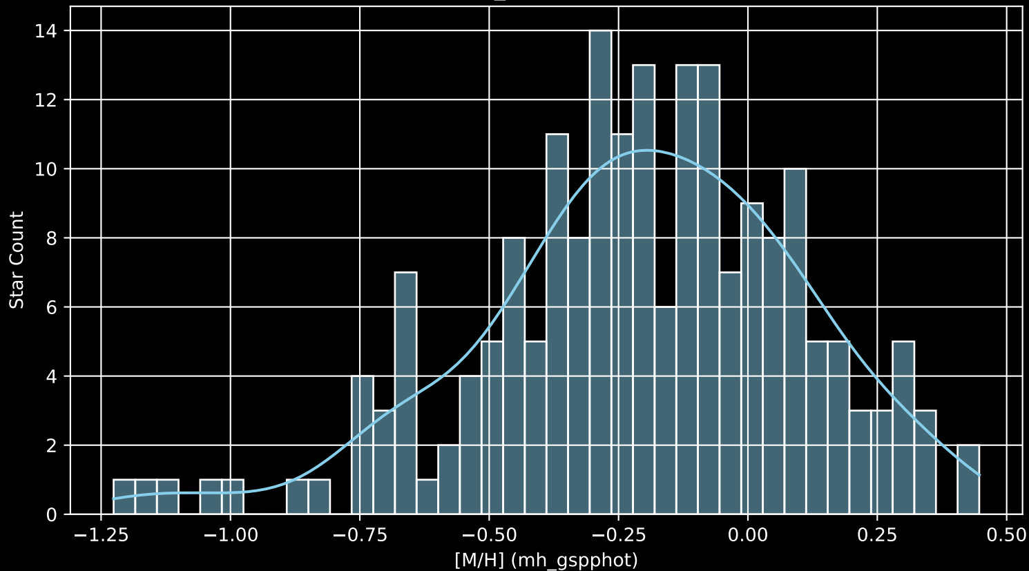
APOGEE DR17 Field: [068+51_MGA [M/H] (mh_gspphot) (n= 195)
