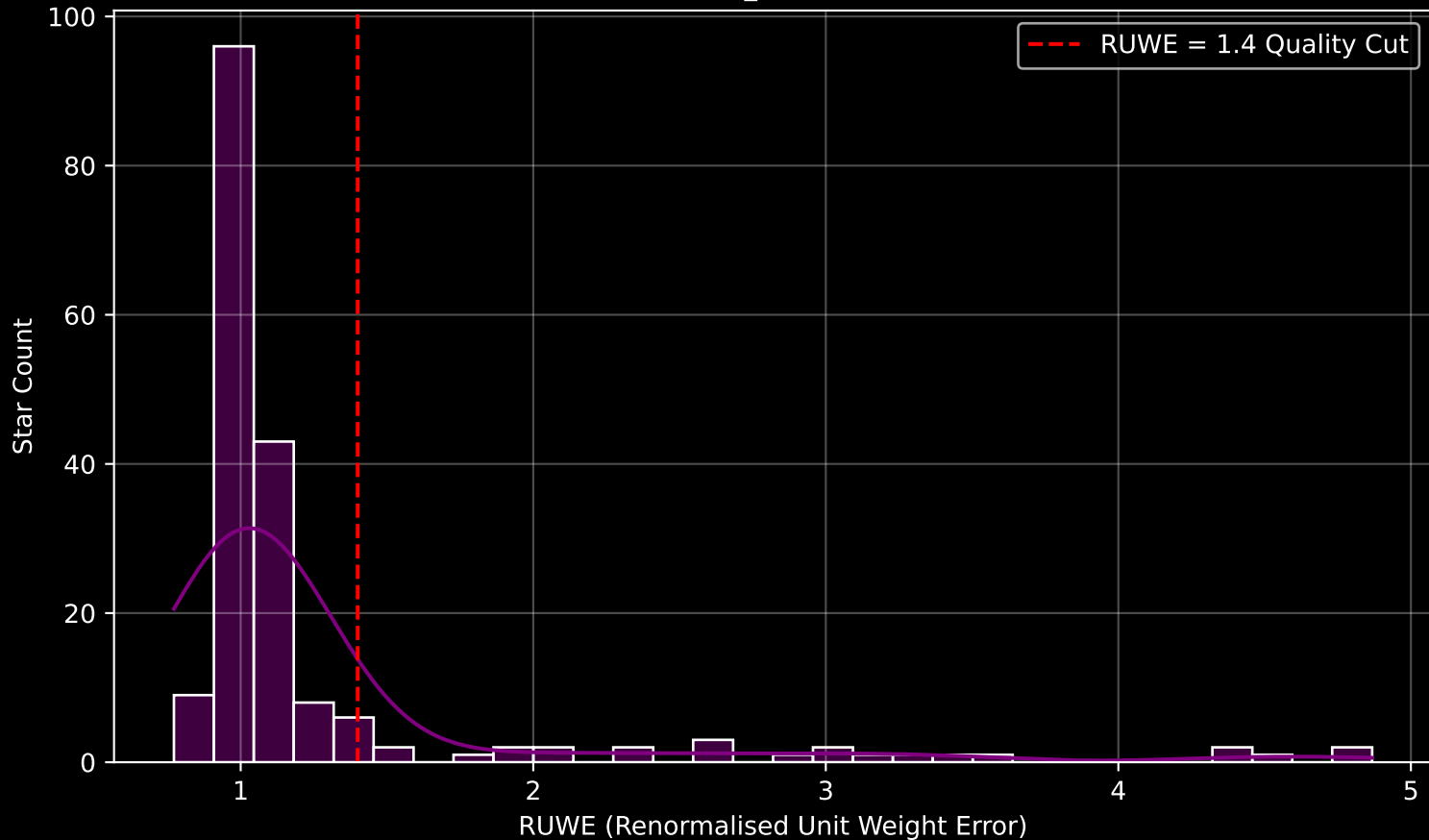
GAPOGEE DR17 Field [068+51_MGA] RUWE Distribution (n= 186)
