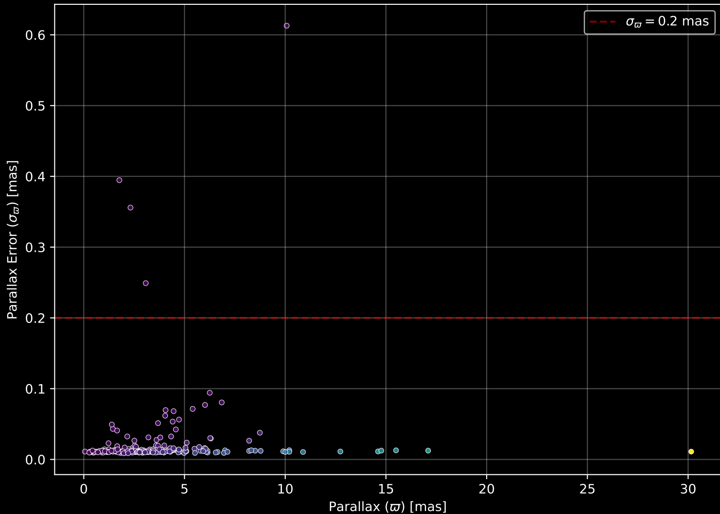
APOGEE DR17 Field: [068+51_MGA] Parallax Quality (n= 197)
