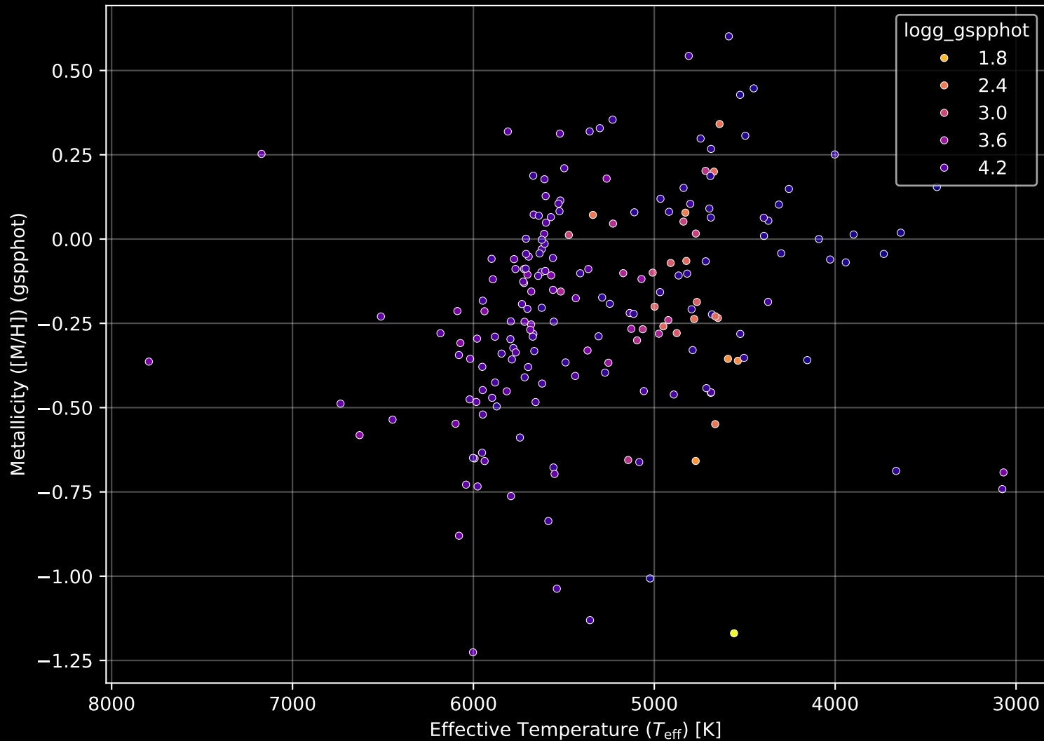
APOGEE DR17 Field: [068+51_MGA] Stellar Population Parameters (n= 197)
